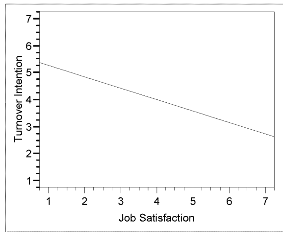
Figure 11: Regression of Turnover Intention by Job Satisfaction
